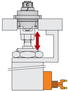
ELECTRICAL CYLINDER
